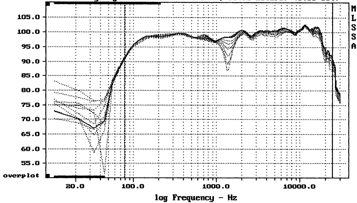
Sensitivity Mag - dB SPL/watt (4 ohms, @1.70 meters) (0.33 oct)
